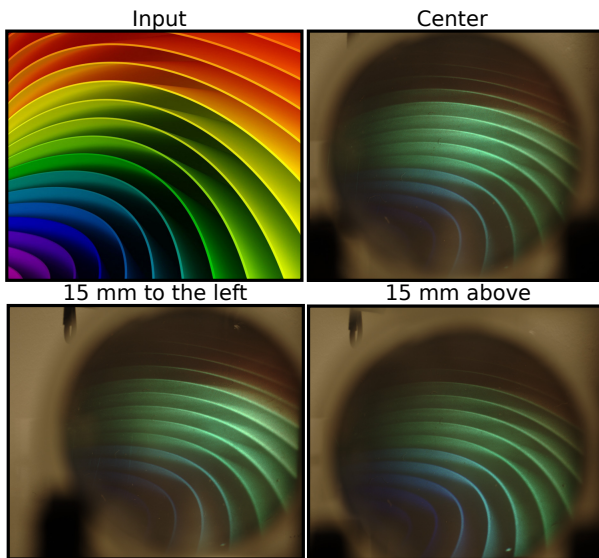
Fig. 10. Examination of eyebox stability. Top left: an input image provided to our light engine. Top right: A photograph taken from the center of our prototype's eyebox. Bottom left: A photograph taken from 15 mm to the left with respect to center of our prototype's eyebox. Bottom right: A photograph taken from 15 mm above the center of our prototype's eyebox.
