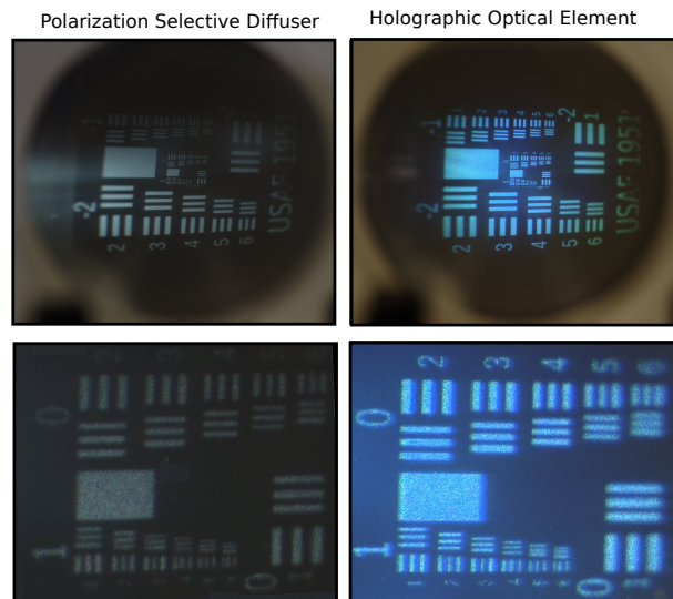
Fig. 8. A pair of photographs showing image quality and visible amount of haze while using (top left) a polarization selective diffuser with anti-reflection coating, and (top right) a holographic diffuser. Bottom row shows magnified central regions of top row.
