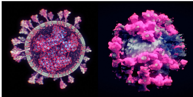
Fig. 8. 3D visualization of a coronavirus particle (Nguyen et al., 2021).
