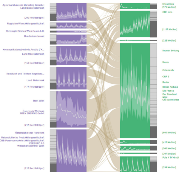
Fig. 14. BiCFlows (Steinböck et al., 2018; Waldner et al., 2020) support the exploratory analysis of very large, time-dependent bipartite graphs, such as media-advertisement networks.
