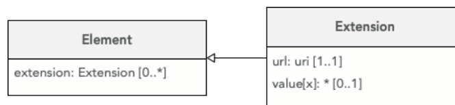
Figure 3.9: UML diagram - FHIR Extension [26]
