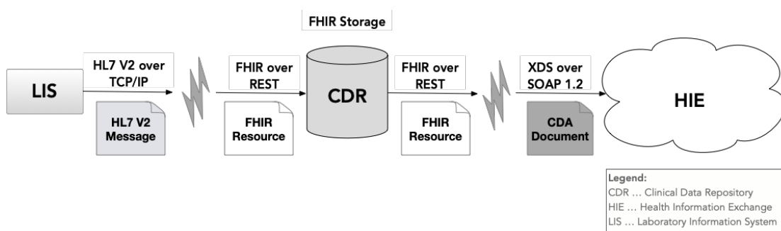
Figure 3.1: Interoperability problems of the connection between the laboratory and the HIE
