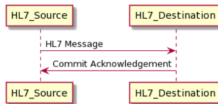
Figure 3.4: HL7 communication over MLLP [17]
