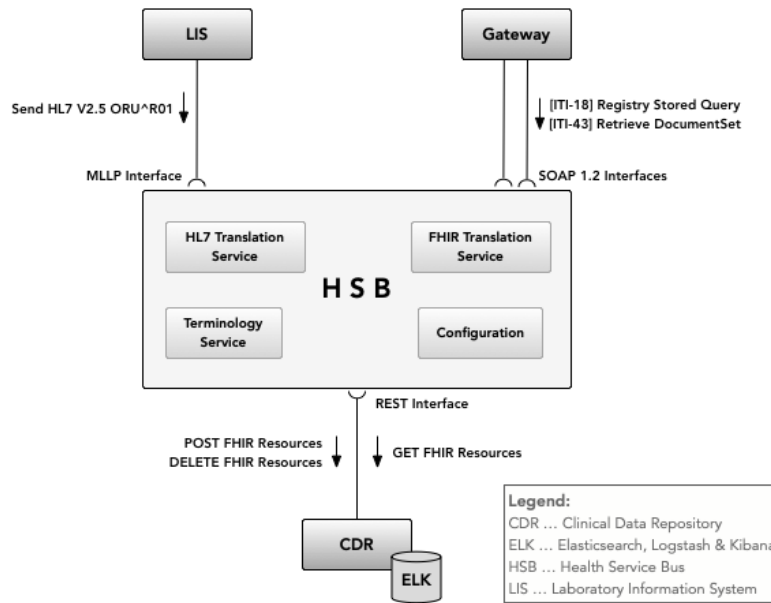
Figure 4.2: Interfaces of the HSB
