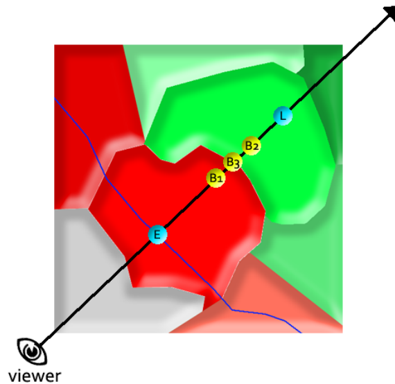
Figure 3.12: Ray tracing performing a binary search to find the cell's boundary. Inside cells are colored green, intersected cells are colored red and outside cells are colored gray. The blue line represents the basic mesh's surface. Three iterations B_1, B_2 and B_3 are needed to hit exactly the inside cell's border.
