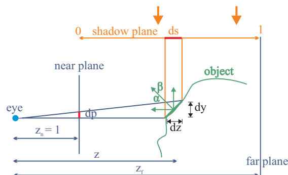
Figure 3: Aliasing in shadow mapping.
