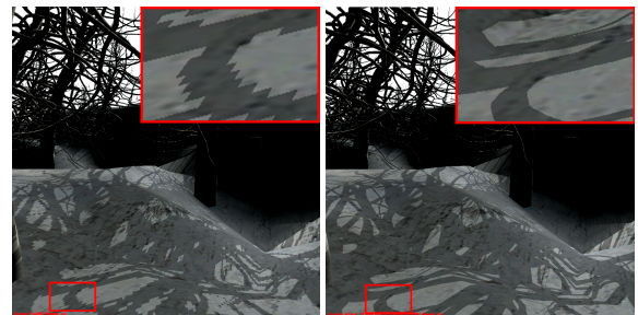
Figure 15: Left: standard 4096 2 shadow map. Right: QVSM with a maximum refinement level of 32x32, and 2048 2 tiles.
