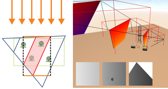
Figure 12: PSSM: Left: The shadow map for the middle of three partitions of the view frustum (side view) is emphasized. Right: The bounding volumes for the partitions are shown in 3D. Inlays show the shadow maps.
