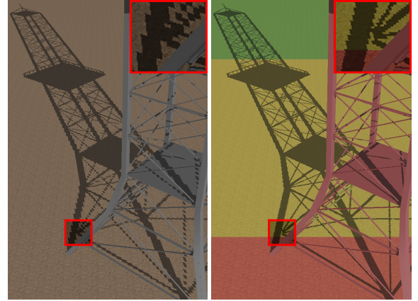
Figure 14: For cases where the light is coming from behind, warping (left) gives unsatisfactory results, while z-partitioning (right) provides superior results. The shadow map used for each fragment is color coded.
