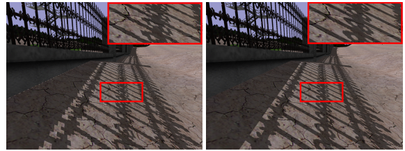
Figure 19: LiSPSM gives good results for a shadow map resolution of 1024^2 and a viewport of 1680 \times 1050 , but temporal reprojection can still give superior results because it is not limited by the shadow map resolution.
