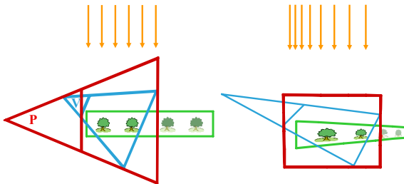
Figure 9: An example configuration of light space perspective shadow maps with view frustum V and the frustum defining the perspective transform P . Left: directional light, a view frustum V , and the perspective transform P . Right: after the warp, objects near the viewer appear bigger in the shadow map and therefore receive more samples.
