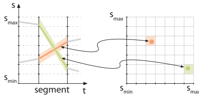
Figure 4: This figure illustrates the duality between bins in a binmap and function graph segments in the corresponding function graph space.
