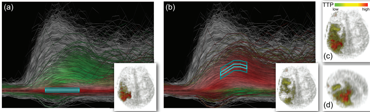
Figure 9: A feature set containing two different features has been defined in two function graph visualizations. In (a), a smooth similarity brush (blue) has been defined such that tissue with no significant signal enhancement is selected in the first feature (shown in its 3D context in the inlet). In (b), a similarity brush has been used to specify a second feature representing tissue exhibiting reduced and delayed perfusion. Candidate areas of this tissue at risk are revealed around the core (inlet). In (c) and (d) the overall feature set is visualized. The color is modified according to the time it takes until the maximum amount of contrast agent is delivered for a particular voxel (TTP).
