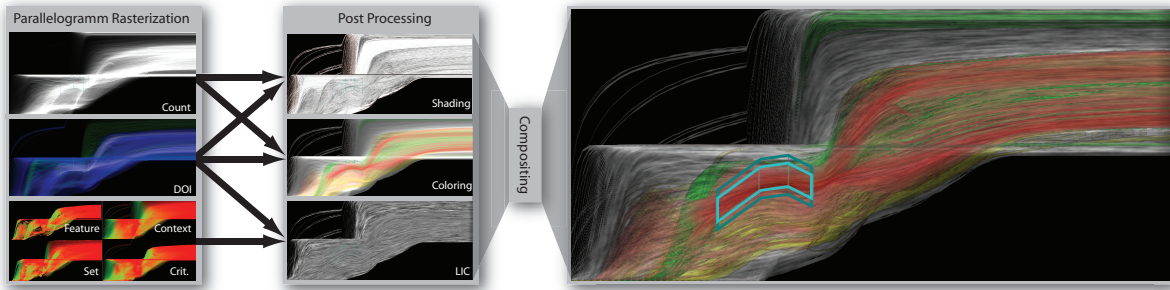
Figure 3: The first stage of our rendering pipeline rasterizes parallelograms (each representing multiple function graph segments) and generates multiple output images which are used by the post processing stage. Here different image based algorithms are applied in order to create three different effects (shading, coloring, and LIC), which are combined in the compositing stage.
