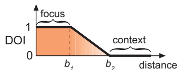
Figure 7: Computing smooth DOI values based on distance values by linearly interpolating between two thresholds.
