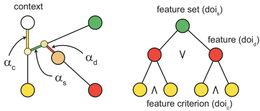
Figure 1: The structure of the FDL tree (right) and the optimized blending scheme for color coding (left). The three colors represent different levels of the FDL tree.
