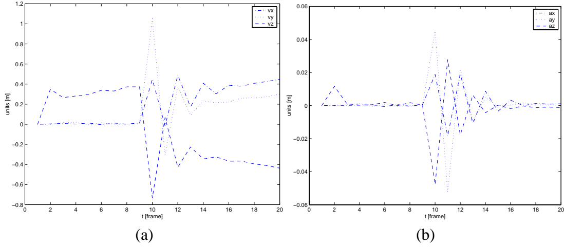
Figure 5.14: Prediction of translational velocity and acceleration. (a) Translational velocity (b) Translational acceleration. It can be seen that translational velocity and -acceleration are more sensitive to noise than angular velocities. The filter is stable only after frame 13.
