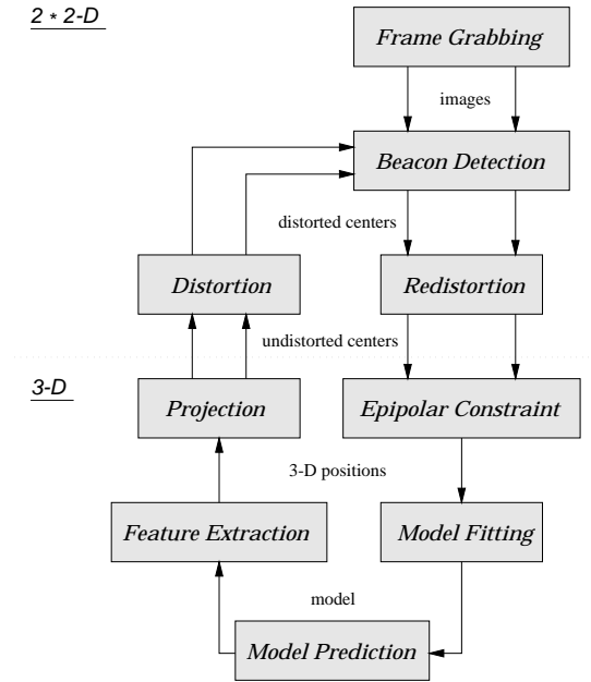
Figure 6.7: The image processing pipeline
