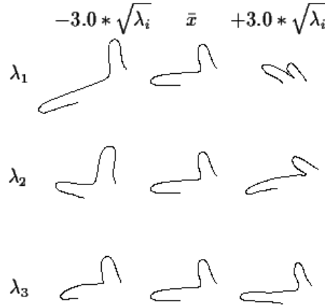
Figure 6.32: The first three modes of variation
