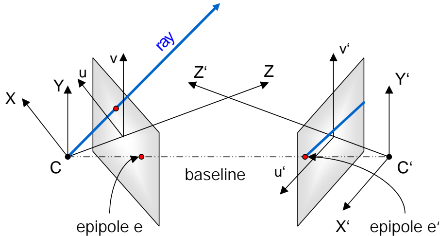
Figure 4.9: The epipolar line
