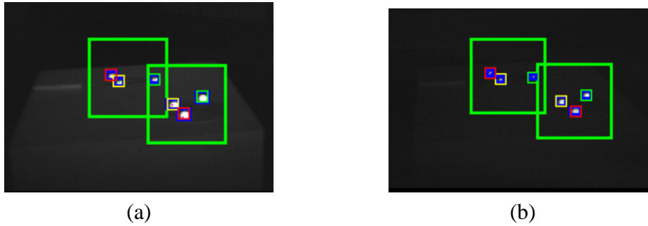
Figure 6.15: Rigid-body identification
