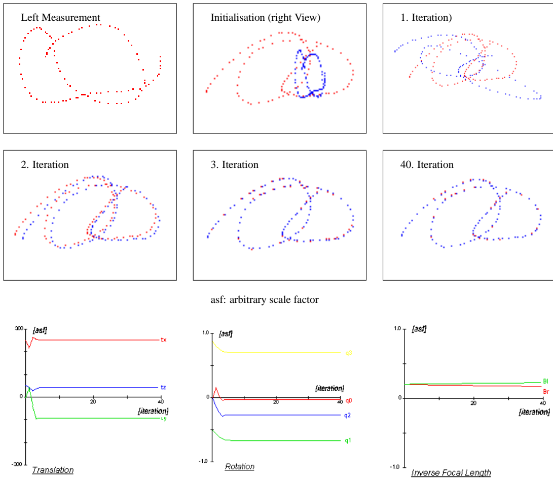
Figure 4.16: The iterative calibration
