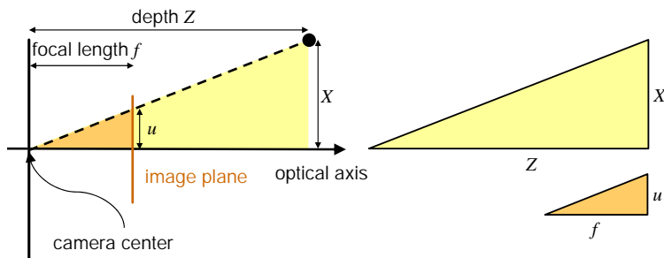
Figure 4.4: Similar triangles of a pinhole camera model
