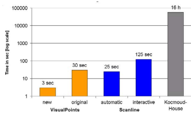
(a) Run Time Comparison
