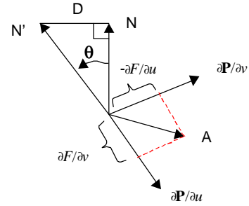
Figure 3. Interpreting a perturbation as a rotation.
