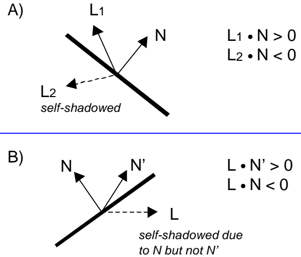
Figure 4. Self-shadowing situations.
